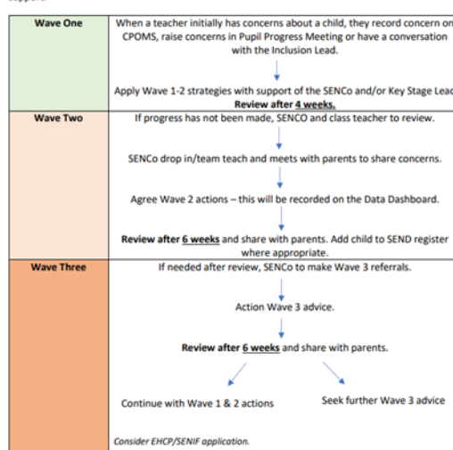
Inclusion Flowchart
